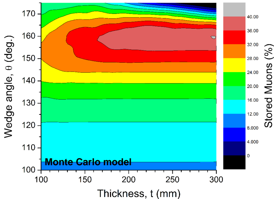
Beryllium, Q=104.0
