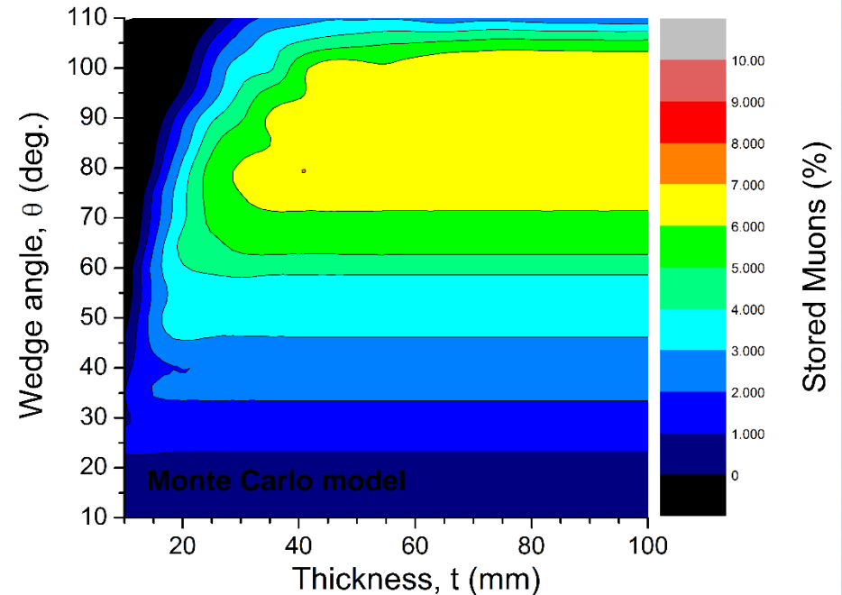
Nickel, Q=18.6
