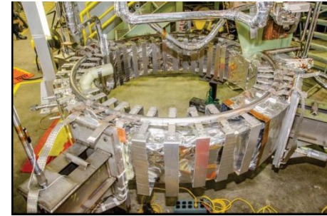
focus coil
