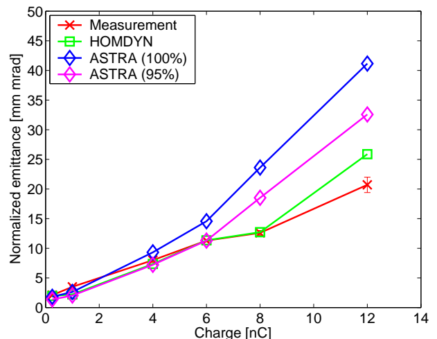
FIG. 2: Comparison of the measured and simulated minimum normalized vertical emittance at z = 3.8 m as a function of the charge per bunch.
