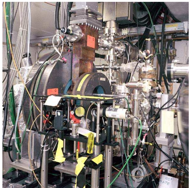
FIG. 1: The Fermilab RF gun. A small optical table for transport of the laser beam can be seen in the foreground, with the iron yokes for the three solenoids behind it. The waveguide feed for the RF gun is between the primary and secondary solenoids. The first two diagnostic ports of the beam line are to the right of the secondary solenoid; the edge of the cryostat for the 9-cell cavity is at the far right.
