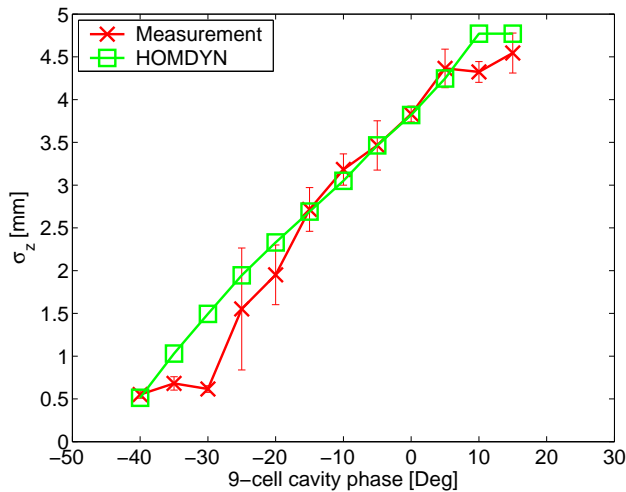
FIG. 5: Measured and simulated compression of a 8 nC beam as a function of the 9-cell cavity phase. The \phi_s = 0 corresponds to acceleration on crest.
