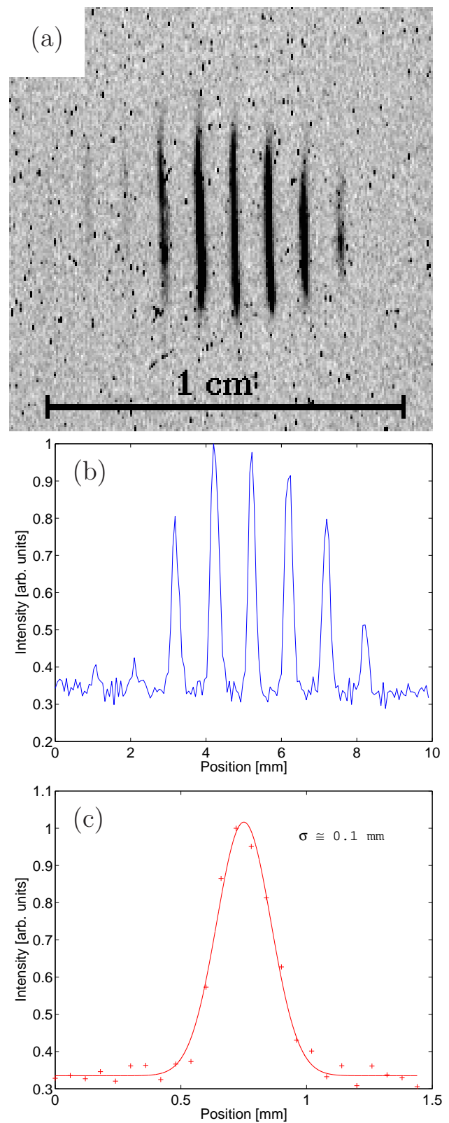
FIG. 3: (a) Image of an 8 nC beam going through the slit mask located 384 mm upstream, (b) density projection, and (c) Gaussian fit of the beamlet of highest intensity.
