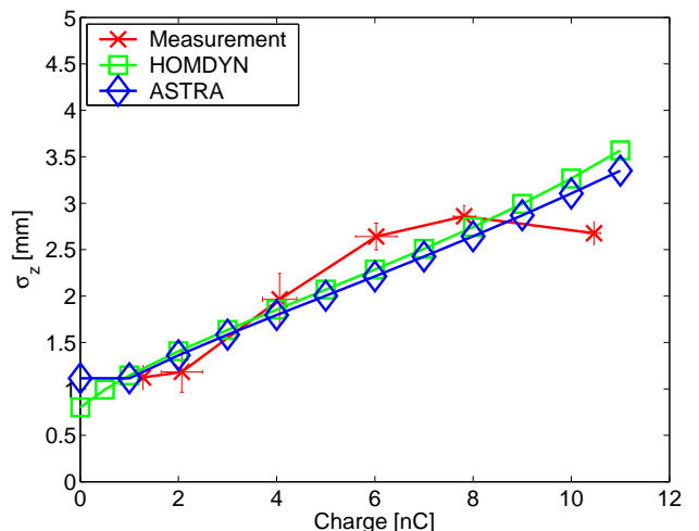
FIG. 4: Comparison of the measured and simulated bunch length as a function of the charge per bunch.
